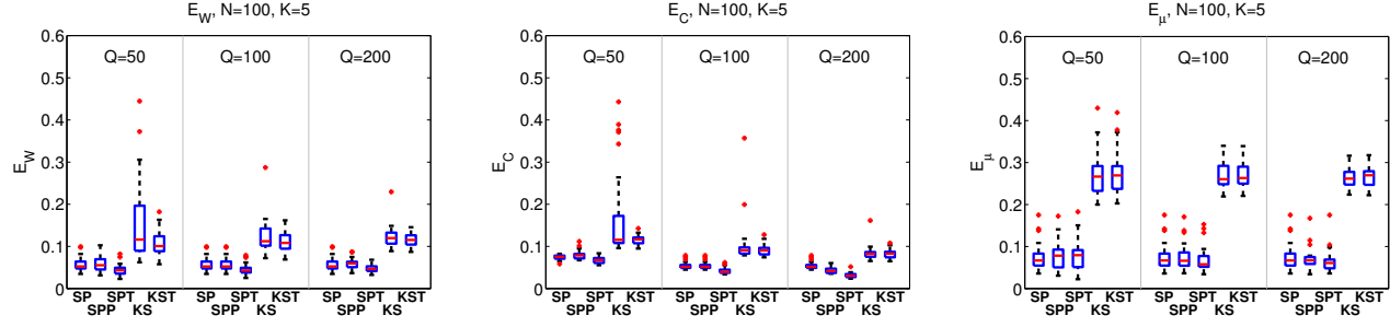
(b) Impact of the number of questions, Q \in \{50, 100, 200\} , with the number of learners N fixed.
