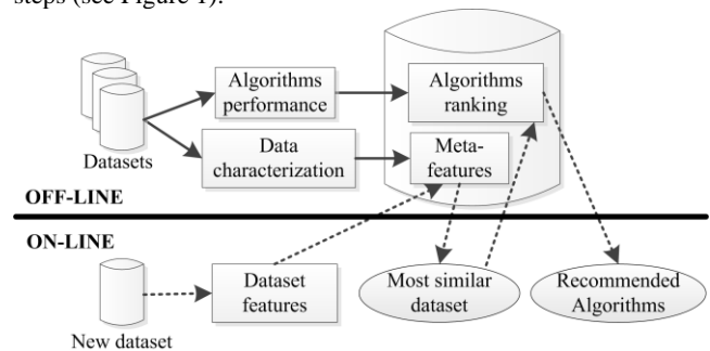
Figure 1. Meta-learning methodology.
