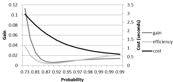
Figure 7. Optimality function.
