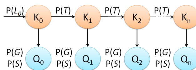
Figure 2. Static Bayesian network representation of Knowledge Tracing
