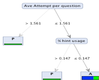
Figure 1. J48 Decision Tree for predicting MCAS classification using data from August through October.
