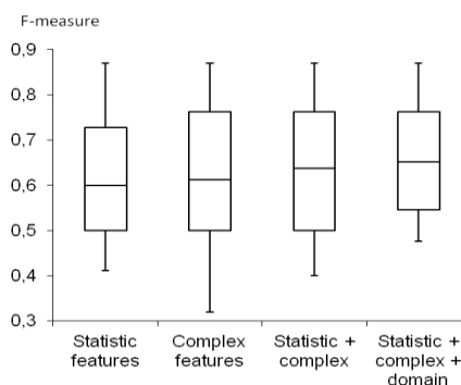
Figure 2. Box plot of the F-measure.
