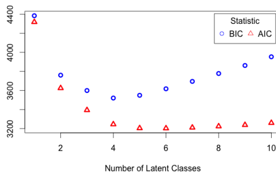
Figure 3: AIC and BIC over increasing number of clusters. BIC bottoms out and AIC levels off at four clusters, so we conclude that four clusters best fits the data.
