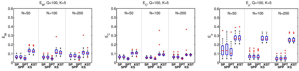
(a) Impact of the number of learners, N \in \{50, 100, 200\} , with the number of questions Q fixed.
