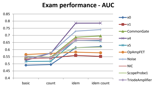
Figure 7. Individual model performance on each exam problem.
